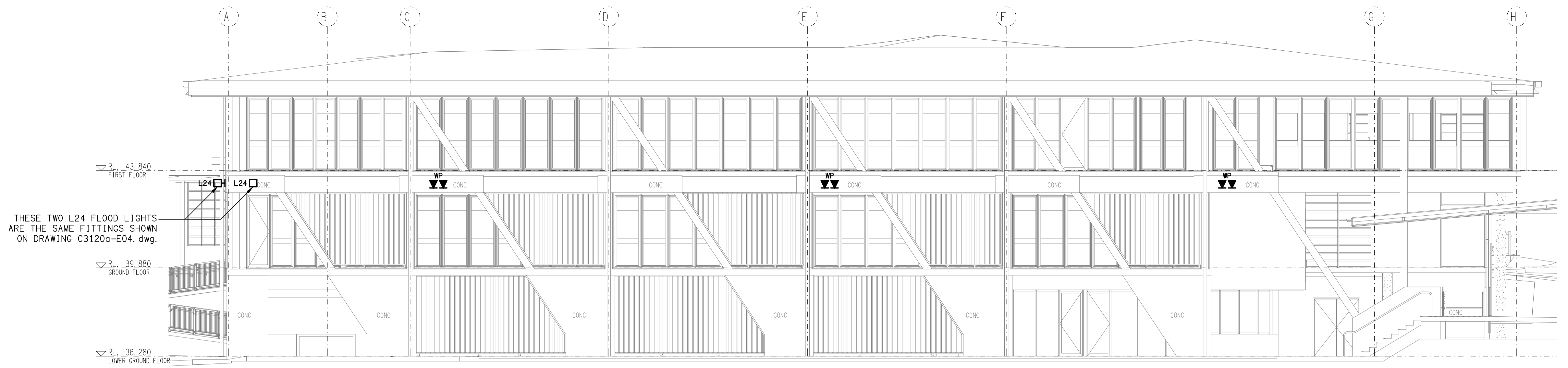
NORTH EXTERNAL BUILDING ELEVATION SCALE 1:100
